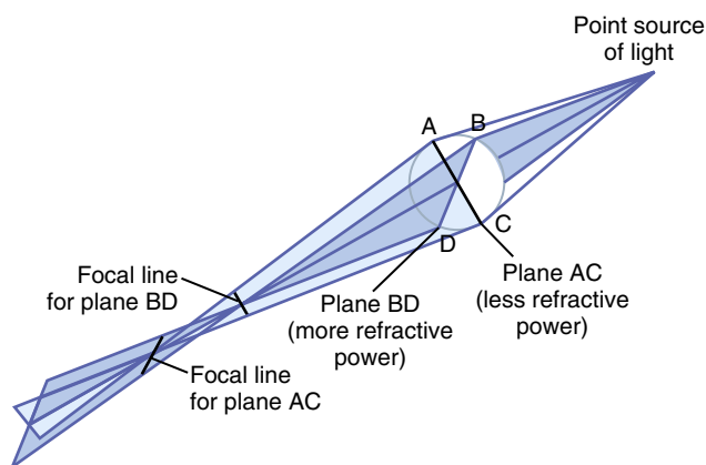
Figure 50-14. Astigmatism, demonstrating that light rays focus at one focal distance in one focal plane ( plane AC ) and at another focal distance in the plane at a right angle ( plane BD ).
