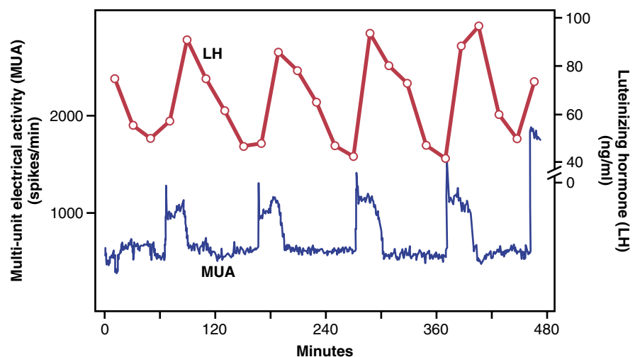
Figure 82-10. Shown is a pulsatile change in luteinizing hormone (LH) in the peripheral circulation of a pentobarbital-anesthetized ovariectomized rhesus monkey (red line) and a minute by minute recording of multi-unit electrical activity (MUA) in the mediobasal hypothalamus (blue line). (Data from Wilson RC, Kesner JS, Kaufman JM, et al: Central electrophysiologic correlates of pulsatile luteinizing hormone secretion . Neuroendocrinology 39:256, 1984.)
