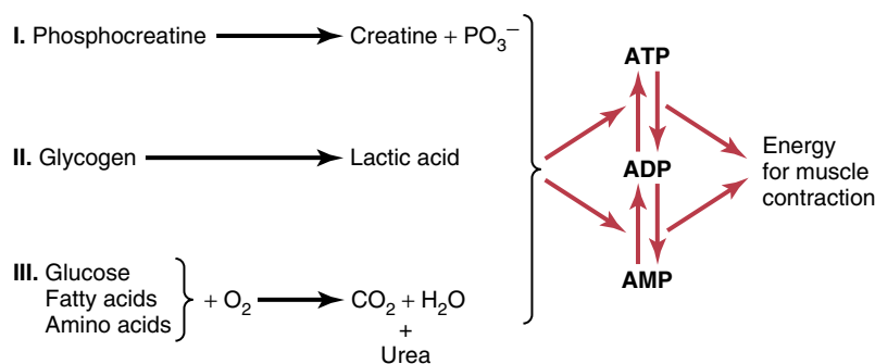
Figure 85-2 Important metabolic systems that supply energy for muscle contraction.
