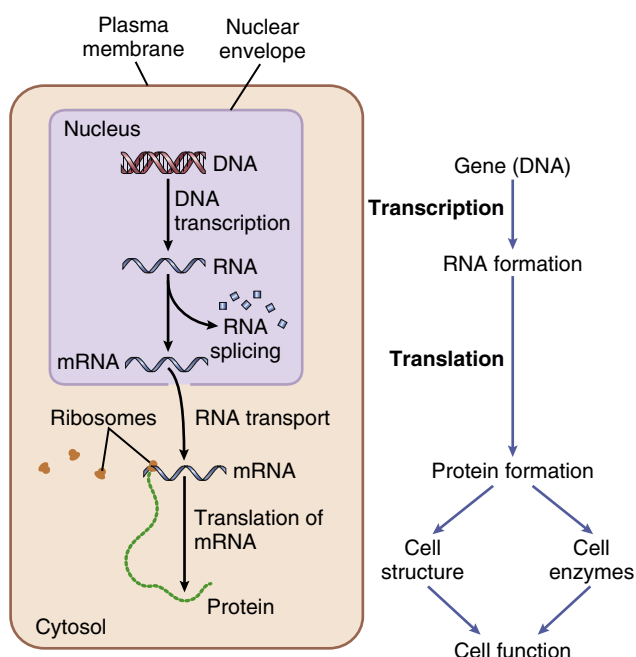
Figure 3-1 The general schema whereby genes control cell function. mRNA, Messenger RNA.
