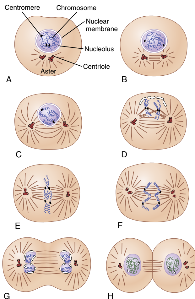
Figure 3-14. Stages of cell reproduction. A, B, C, Prophase. D, Prometaphase. E, Metaphase. F, Anaphase. G, H, Telophase.
