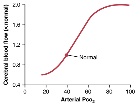
Figure 62-2. Relationship between arterial \text{PCO}_2 and cerebral blood flow.
