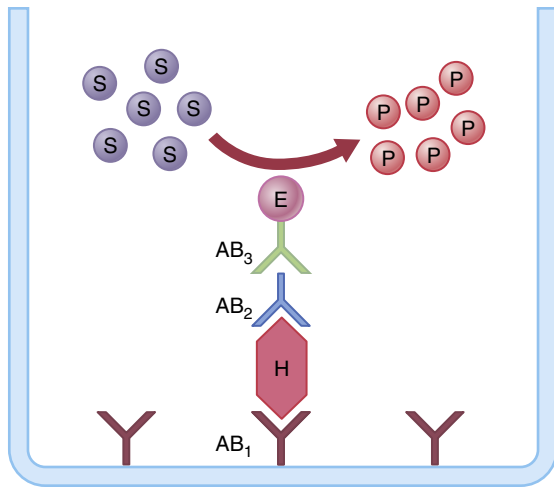
Figure 75-10. Basic principles of the enzyme-linked immunosorbent assay for measuring the concentration of a hormone ( H ). AB 1 and AB 2 are antibodies that recognize the hormone at different binding sites, and AB 3 is an antibody that recognizes AB 2 . E is an enzyme linked to AB 3 that catalyzes the formation of a colored fluorescent product ( P ) from a substrate ( S ). The amount of the product is measured using optical methods and is proportional to the amount of hormone in the well if there are excess antibodies in the well.
