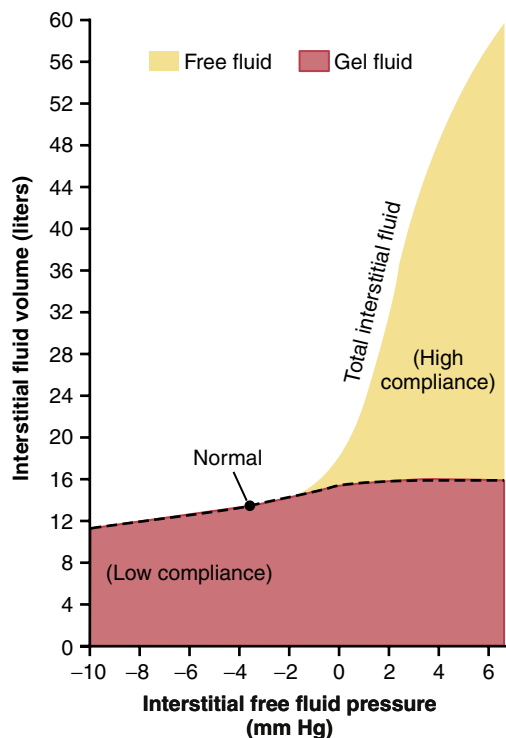
Figure 25-8. Relationship between interstitial fluid hydrostatic pressure and interstitial fluid volumes, including total volume, free fluid volume, and gel fluid volume, for loose tissues such as skin. Note that significant amounts of free fluid occur only when the interstitial fluid pressure becomes positive. (Modified from Guyton AC, Granger HJ, Taylor AE: Interstitial fluid pressure . Physiol Rev 51:527, 1971.)
