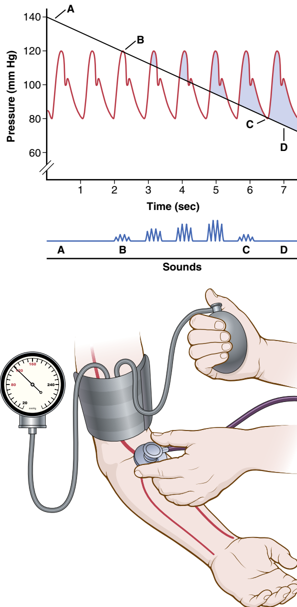
Figure 15-7. Auscultatory method for measuring systolic and diastolic arterial pressures.
