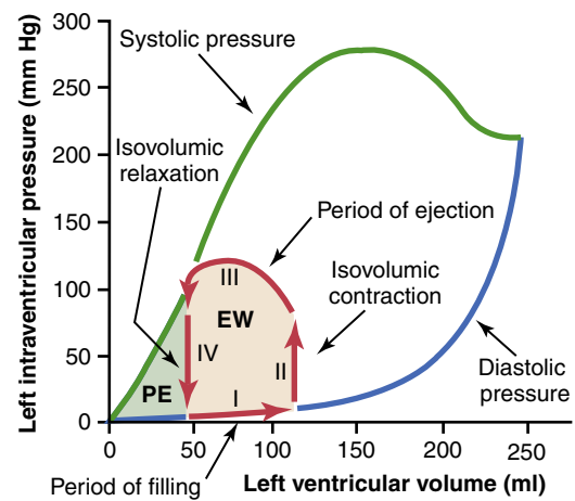
Figure 9-10. Relationship between left ventricular volume and intra-ventricular pressure during diastole and systole. Also shown by the red lines is the “volume-pressure diagram,” demonstrating changes in intraventricular volume and pressure during the normal cardiac cycle. EW, Net external work; PE, potential energy.
