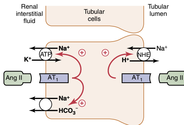
Figure 28-18 Direct effects of angiotensin II ( Ang II ) to increase proximal tubular sodium reabsorption. Ang II stimulates sodium-hydrogen exchange (NHE) on the luminal membrane and \text{Na}^+\text{-K}^+ ATPase transporter as well as sodium-bicarbonate co-transport on the basolateral membrane. These same effects of Ang II likely occur in several other parts of the renal tubule, including the loop of Henle, distal tubule, and collecting tubule. \text{AT}_1 , Angiotensin II type I receptor.
