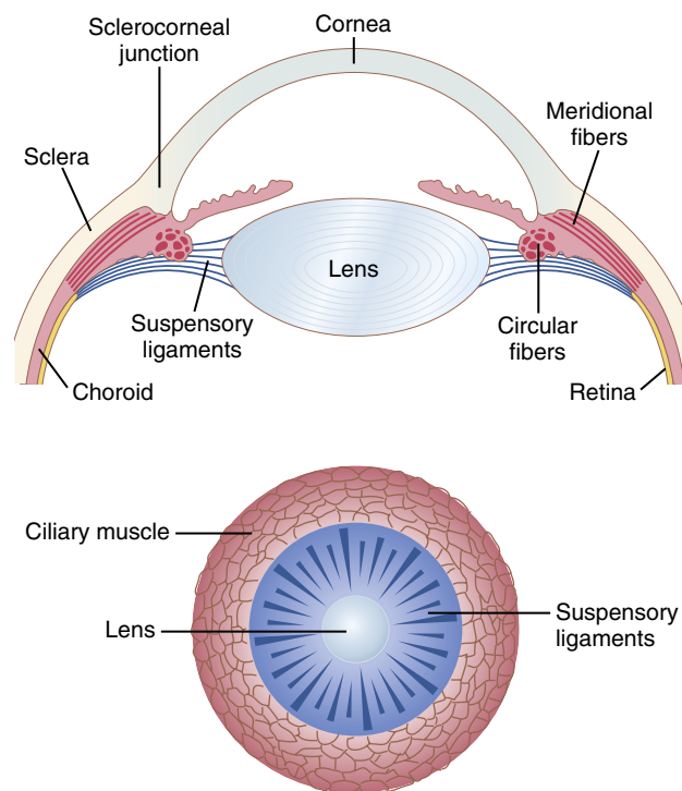
Figure 50-10. Mechanism of accommodation (focusing).
