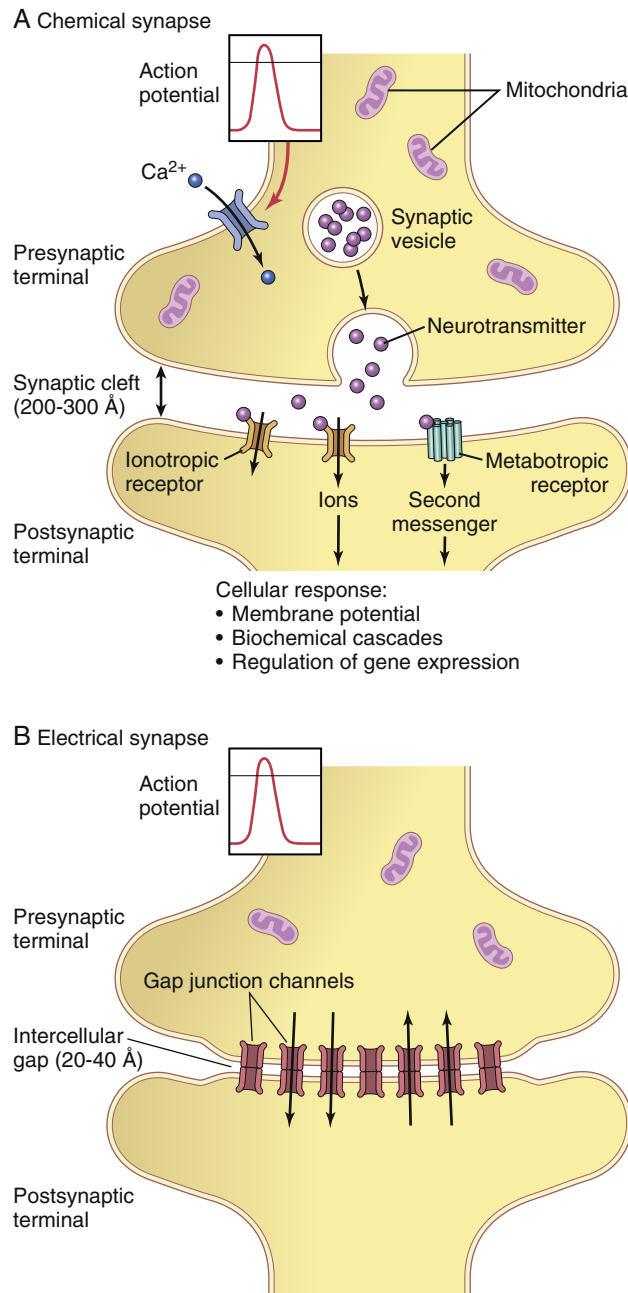
Figure 46-5. Physiologic anatomy of (A) chemical synapse and (B) electrical synapse.
