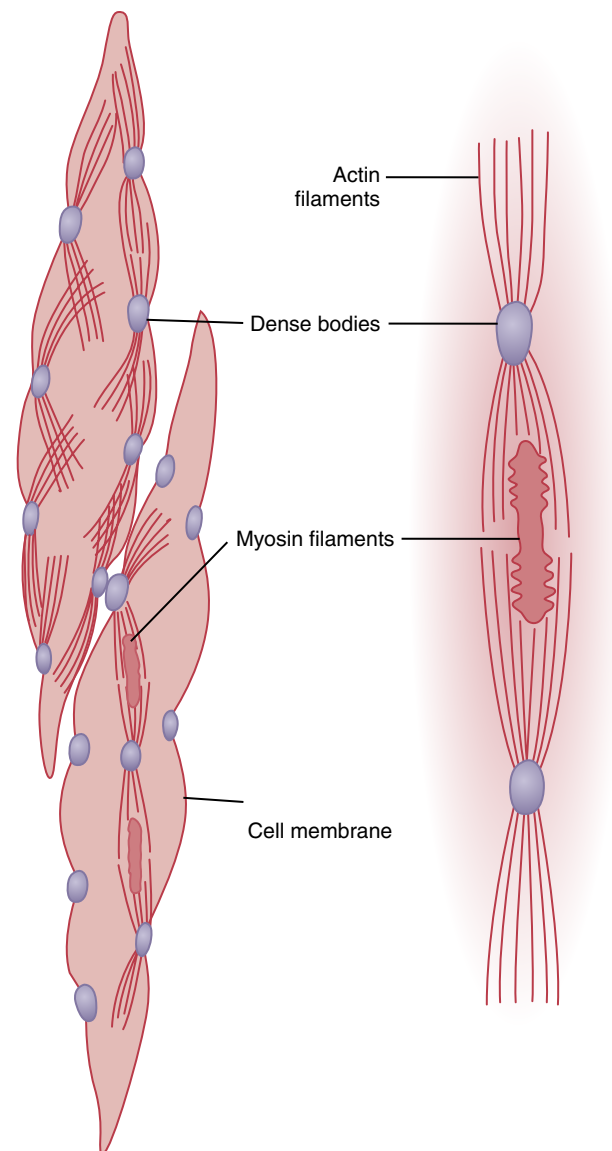
Figure 8-2 Physical structure of smooth muscle. The fiber on the upper left shows actin filaments radiating from dense bodies. The fiber on the lower left and at right demonstrate the relation of myosin filaments to actin filaments.
