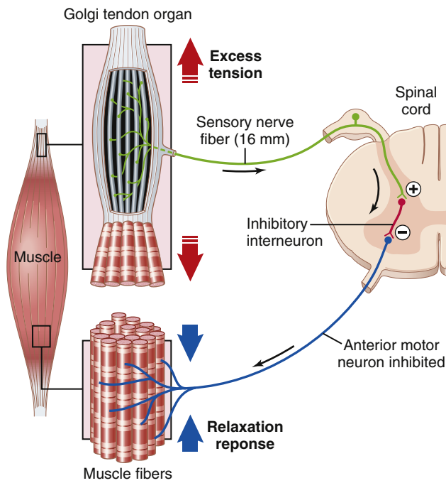
Figure 55-8. Golgi tendon reflex. Excessive tension of the muscle stimulates sensory receptors in the Golgi tendon organ. Signals from the receptors are transmitted through a sensory afferent nerve fiber that excites an inhibitory interneuron in the spinal cord, inhibiting anterior motor neuron activity, causing muscle relaxation, and protecting the muscle against excessive tension.
