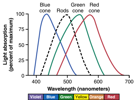
Figure 51-8. Light absorption by the pigment of the rods and by the pigments of the three color-receptive cones of the human retina. (Data from Marks WB, Dobelle WH, MacNichol EF Jr: Visual pigments of single primate cones. Science 143:1181, 1964; and Brown PK, Wald G: Visual pigments in single rods and cones of the human retina: direct measurements reveal mechanisms of human night and color vision. Science 144:45, 1964.)
