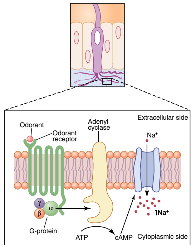
Figure 54-4. Summary of olfactory signal transduction. Binding of the odorant to a G-protein-coupled receptor causes the activation of adenylate cyclase, which converts adenosine triphosphate (ATP) to cyclic adenosine monophosphate (cAMP). The cAMP activates a gated sodium channel that increases sodium influx and depolarizes the cell, exciting the olfactory neuron and transmitting action potentials to the central nervous system.
