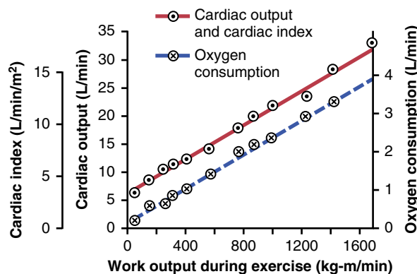
Figure 20-3. Effect of increasing levels of exercise to increase cardiac output (red solid line) and oxygen consumption (blue dashed line). (Modified from Guyton AC, Jones CE, Coleman TG: Circulatory Physiology: Cardiac Output and Its Regulation , 2nd ed. Philadelphia: WB Saunders, 1973.)
