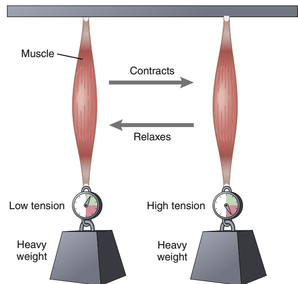
Figure 6-12 Isotonic and isometric systems for recording muscle contractions. Isotonic contraction occurs when the force of the muscle contraction is greater than the load, and the tension on the muscle remains constant during the contraction. When the muscle contracts, it shortens and moves the load. Isometric contraction occurs when the load is greater than the force of the muscle contraction; the muscle creates tension when it contracts, but the overall length of the muscle does not change.
