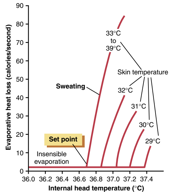
Figure 74-8. Effect of changes in the internal head temperature on the rate of evaporative heat loss from the body (in °C). Note that the skin temperature determines the set point level at which sweating begins. (Courtesy Dr. T.H. Benzinger.)
