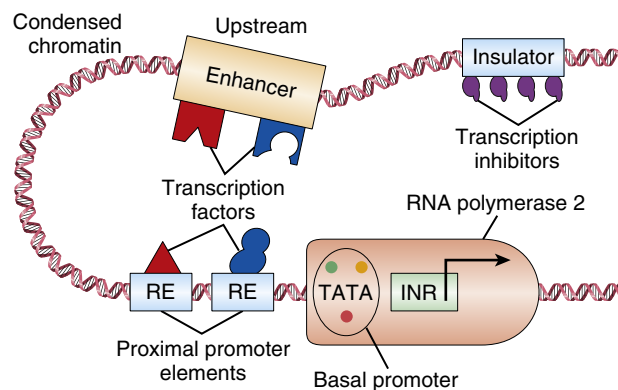
Figure 3-13. Gene transcription in eukaryotic cells. A complex arrangement of multiple clustered enhancer modules is interspersed with insulator elements, which can be located upstream or downstream of a basal promoter containing TATA box (TATA), proximal promoter elements (response elements, RE), and initiator sequences (INR).
