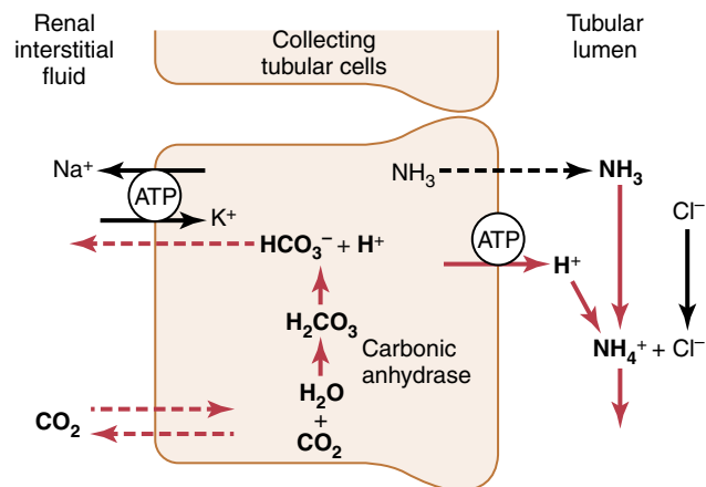
Figure 31-9. Buffering of H + secretion by ammonia (NH 3 ) in the collecting tubules. NH 3 diffuses into the tubular lumen, where it reacts with secreted H + to form NH 4 + , which is then excreted. For each NH 4 + excreted, a new HCO 3 - is formed in the tubular cells and returned to the blood.
